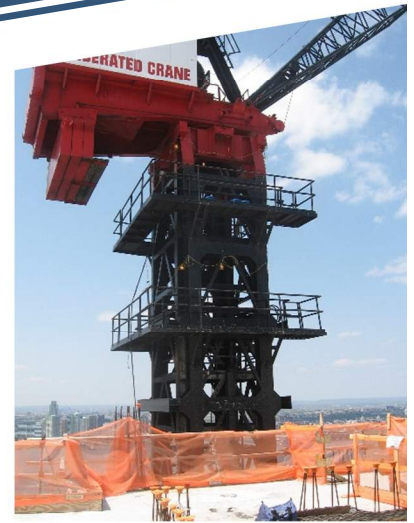
Tower Crane Installations
