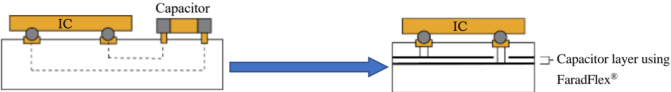
FaradFlex® embedded in a PCB
