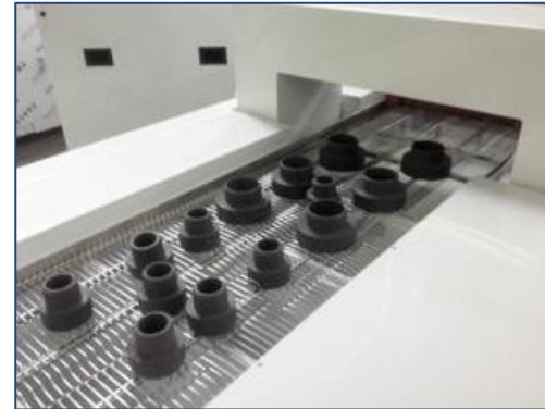
Part passing under the built in demagnetizing unit at the entrance to the Nu/Clean Industrial Cleaner
